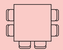
Cluster 30
